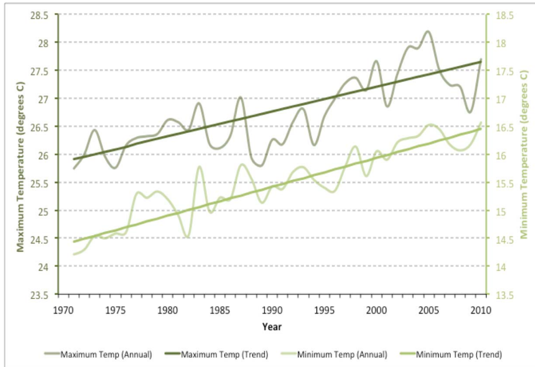
Figure 6: Annual trend in maximum temperature (left-hand axis) and minimum temperature (right-hand axis) for Kigali Airport (1971-2010)
