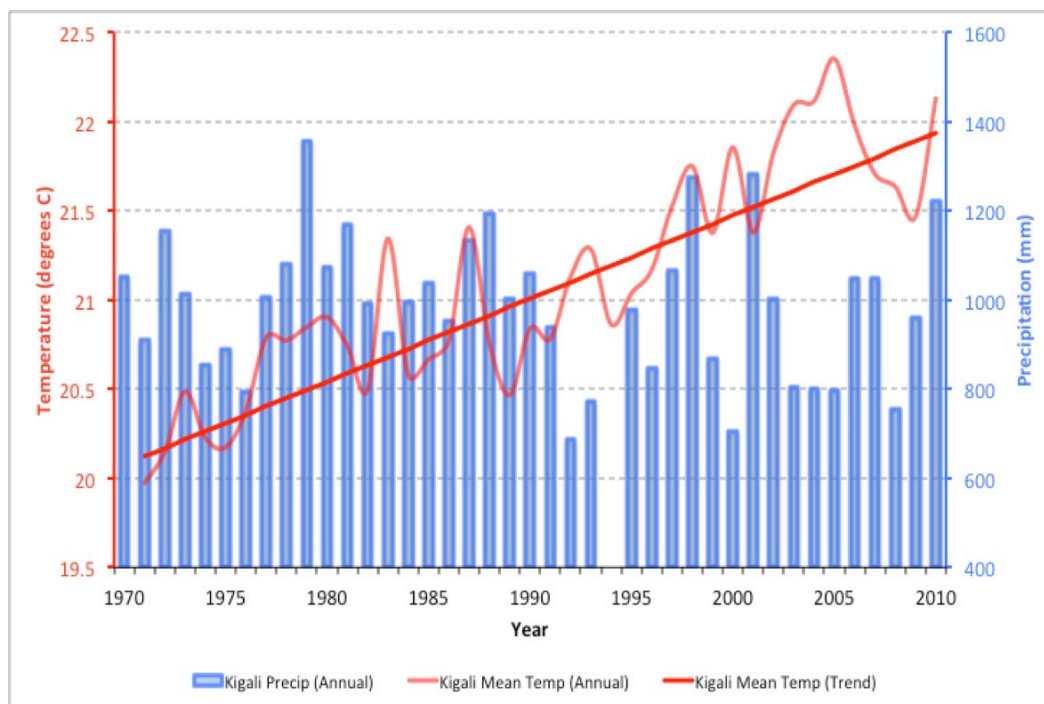
Figure 5: Annual trend in mean temperature (left-hand axis) and precipitation (right-hand axis) for Kigali Airport (1971-2010)
