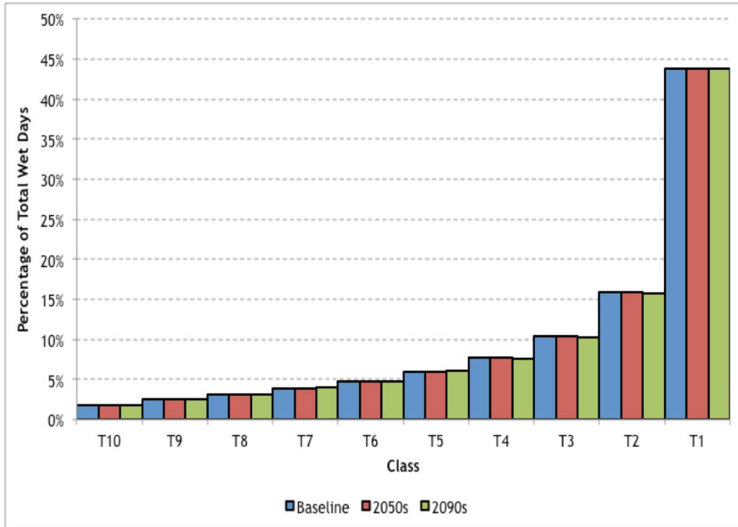
Figure 17: Median projected changes in daily OND rainfall intensity across the ten classes of rainfall. Under A2 SRES scenario for 2050s and 2090s timeslices, against a baseline of 1961-2000; from 10 GCMs of CMIP3, downscaled to Butare station only.
