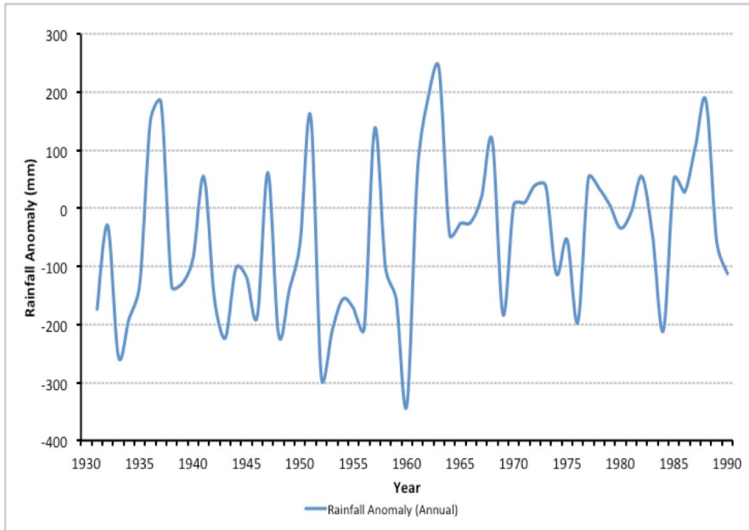
Figure 11: Annual anomaly for precipitation for Rwanda average (1931-90 against a baseline of 1961-90); from 26 stations.
