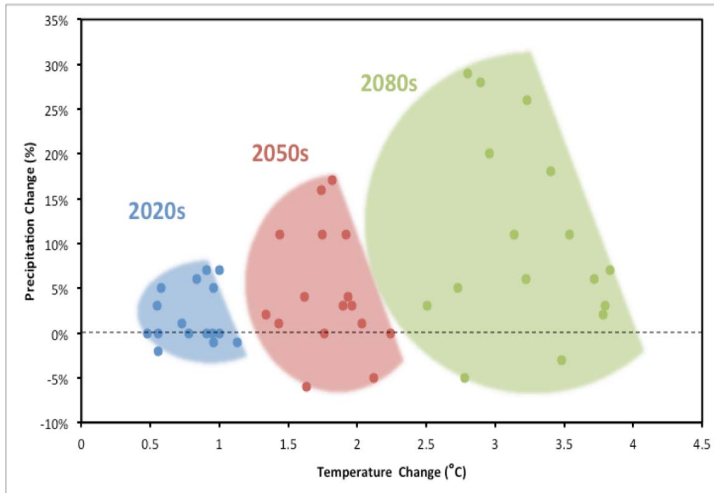
Figure 16: Projected annual change in temperature (degrees C) and precipitation (%) for Rwanda for the 2020s (blue), 2050s (red) and 2080s (green) for the A2 SRES scenario. Dots show individual GCMs; shading indicates spread of results.
