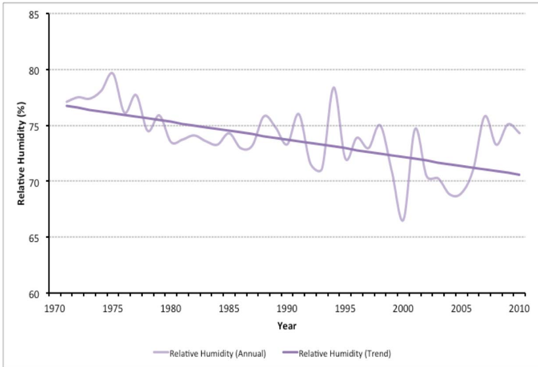
Figure 7: Annual trend in relative humidity for Kigali Airport (1971-2010)
