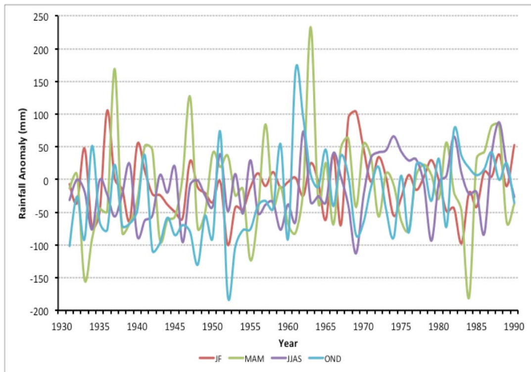
Figure 12: Seasonal anomalies for precipitation for Rwanda average (1931-90 against a baseline of 1961-90); from 26 stations.
