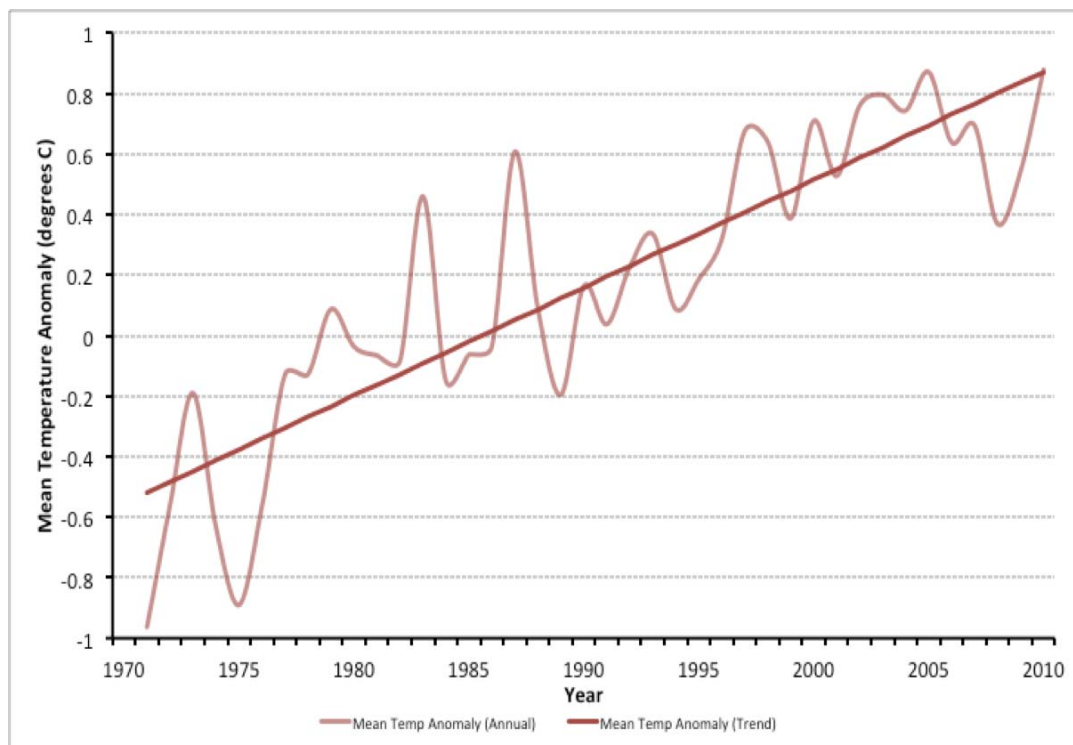
Figure 9: Annual anomaly and trend for mean temperature for Rwanda (1971-2010 against a baseline of 1971-2000); from 4 stations.
