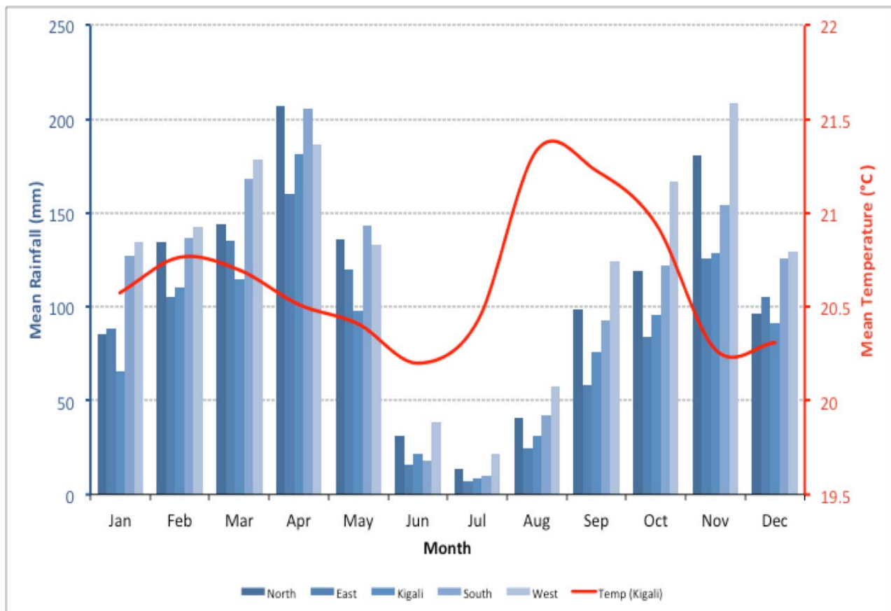
Figure 1: Monthly average rainfall for each region in Rwanda and monthly average temperature for Kigali Aero (1961-90). Stations used: Rulindo (North), Kibungo (East), Kigali Aero (Kigali), Kibeho (South) and Mugonero (West).
