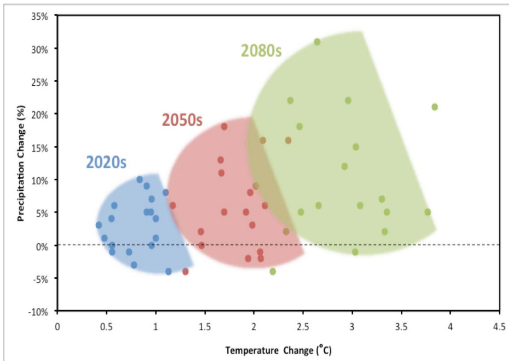
Figure 15: Projected annual change in temperature (degrees C) and precipitation (%) for Rwanda for the 2020s (blue), 2050s (red) and 2080s (green) for the A1B SRES scenario. Dots show individual GCMs; shading indicates spread of results.
