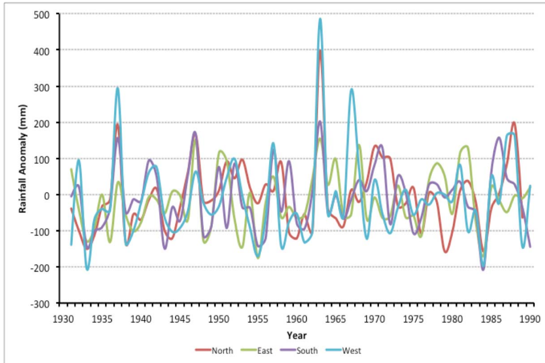
Figure 13: MAM anomalies for precipitation for regions of Rwanda average (1931-90 against a baseline of 1961-90); from 26 stations.
