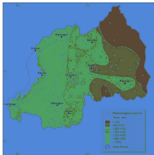
Figure 2: Distribution of rainfall across Rwanda, with annual average total figure Source: Malesu et al., 2010
