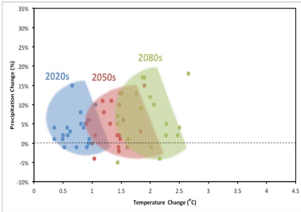
Figure 14: Projected annual change in temperature (degrees C) and precipitation (%) for Rwanda for the 2020s (blue), 2050s (red) and 2080s (green) for the B1 SRES scenario. Dots show individual GCMs; shading indicates spread of results.
