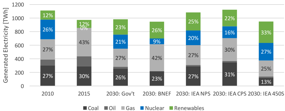
Figure 25: 2030 projections of Japan's electricity mix 84,85,86,87
