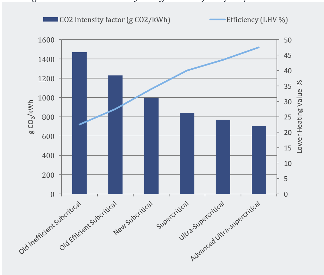
Figure 12: Emissions intensity and efficiencies of coal-fired power stations 40
