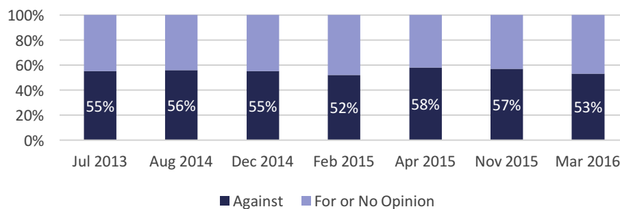
Figure 33: Opposition to nuclear restarts in Japan 163,164
