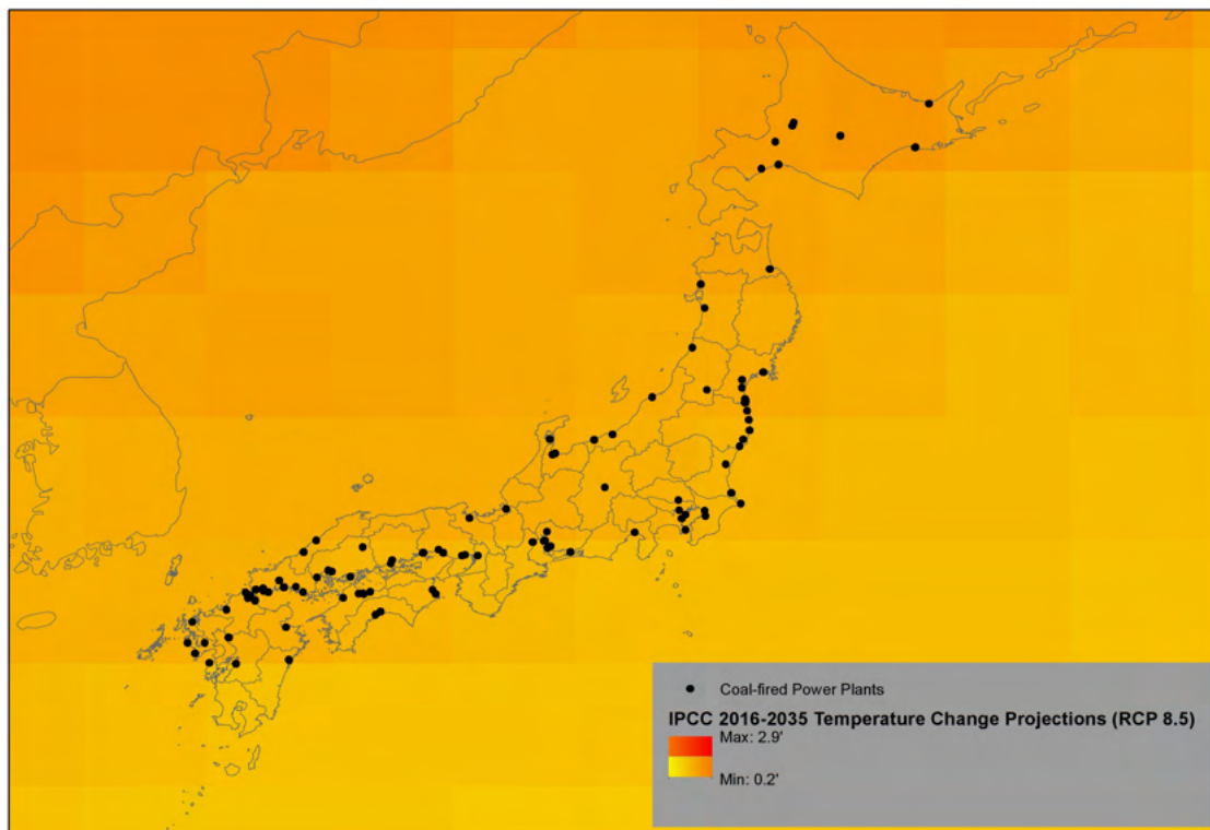
Figure 21: Projected 2016-35 temperature change 73
