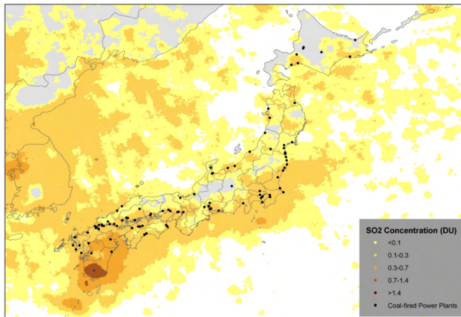
Figure 17: Average SO 2 concentrations, 2011-14 52
