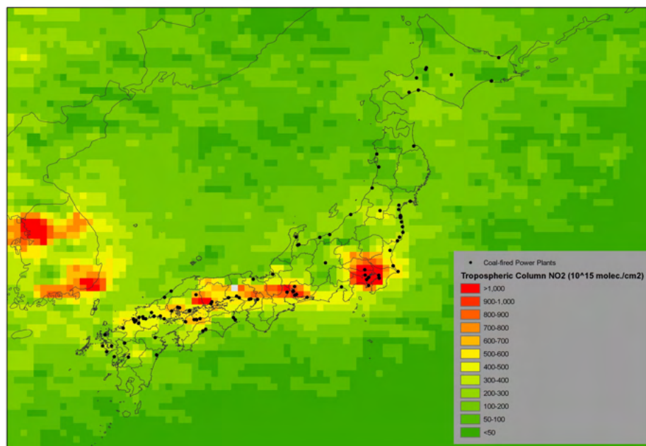
Figure 16: Average NO_2 concentrations, 2015 51
