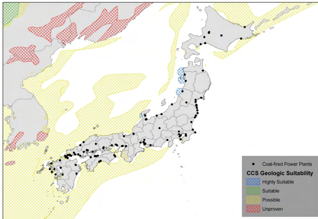
Figure 20: CCS geological suitability 70
