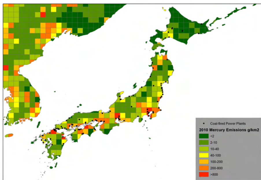
Figure 18: Average mercury emissions, 2010 53
