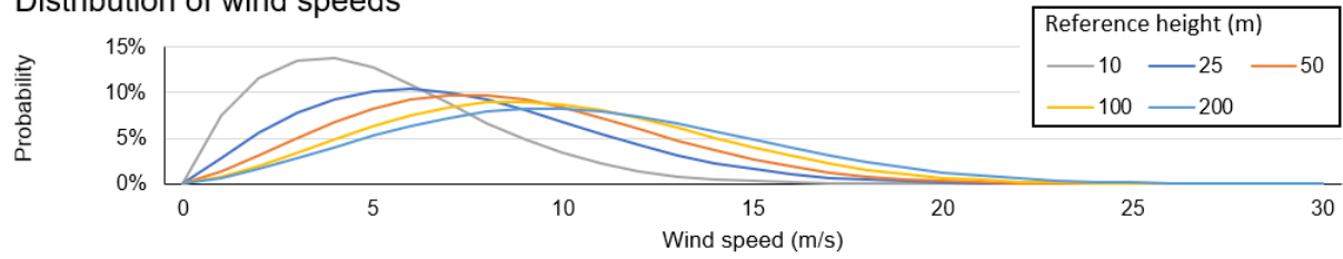
Supplementary Figure 2. Impact of turbine reference height on wind speeds and power outputs.
